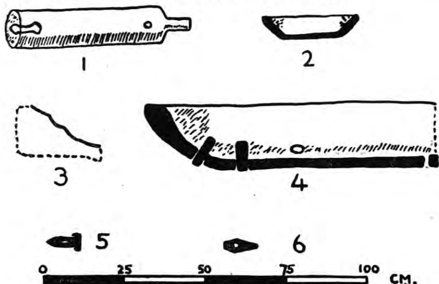
1. Pump, Plakalnica; 2. Wooden bowl, Etropole; 3. Millstone, Etropole; 4. Gradle, Leca; 5. Gad, G. Lom; 6. Gad, Plakalnica.
