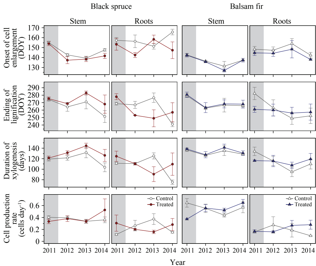
Figure 2.2 Xylem phenology and cell production rate in stem and roots of black spruce and balsam fir during the 4 years of the study. Shaded areas mark the year before thinning.
