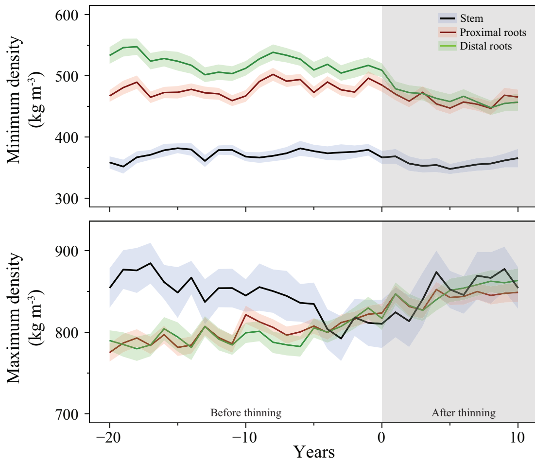
Figure 4.5 Minimum earlywood and maximum latewood density of stem and roots of residual black spruce trees before and after commercial thinning.
