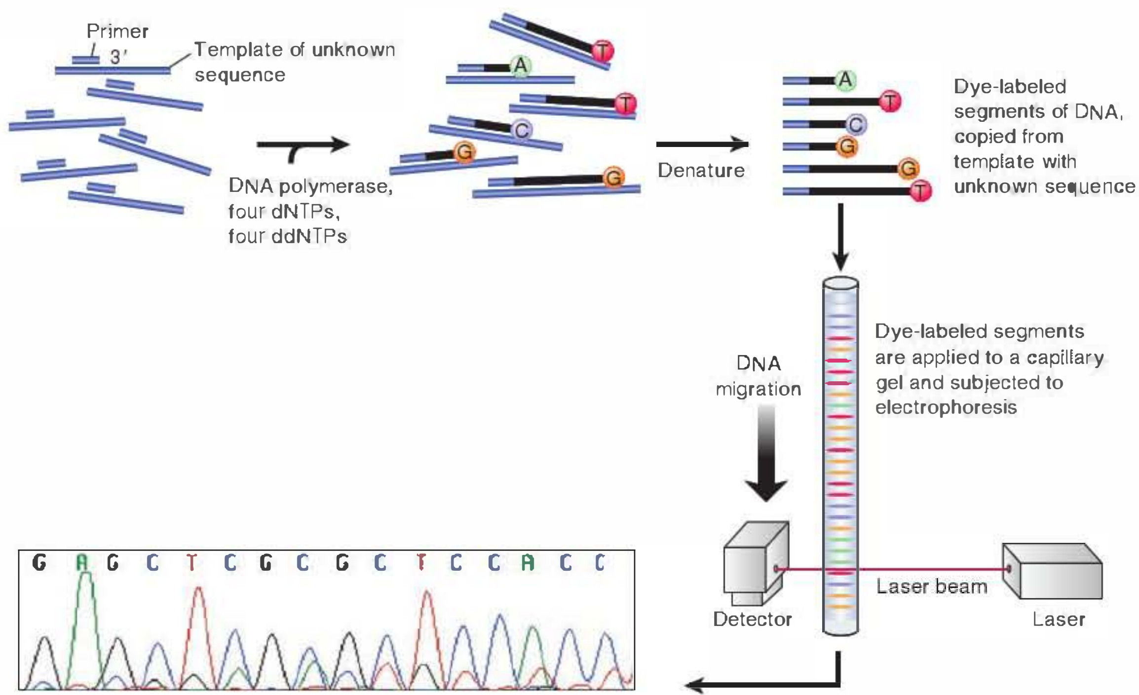
FIGURE 3.17 DideoxyNTP sequencing using fluorescent tags. Inset photo courtesy of Jan Kieleczawa.
