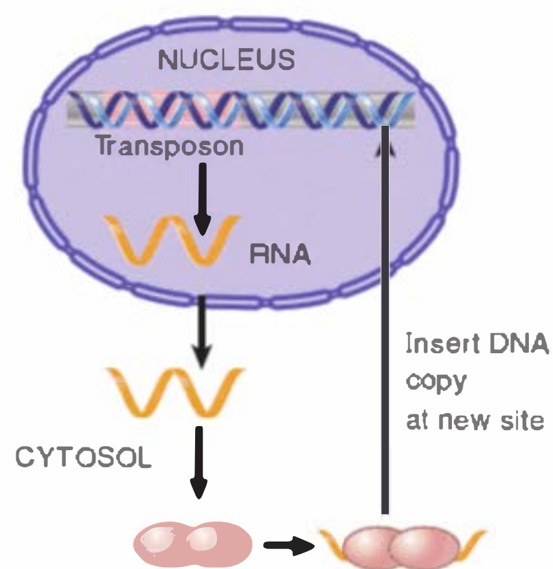
FIGURE 17.37 A LINE is transcribed into an RNA that is translated into proteins that assemble into a complex with the RNA. The complex translocates to the nucleus, where it inserts a DNA copy into the genome.
