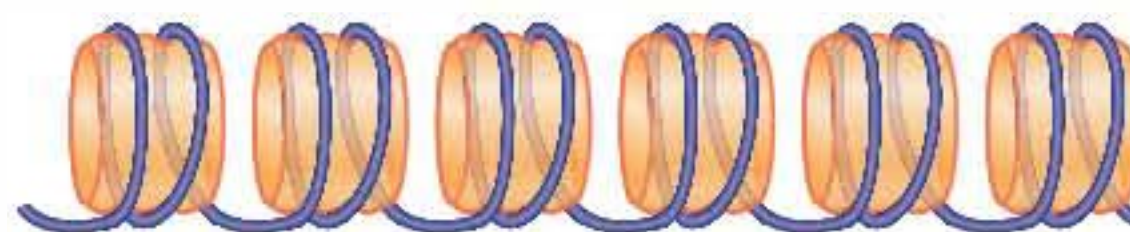
FIGURE 10.32 The 10-nm fiber is a continuous string of nucleosomes.
