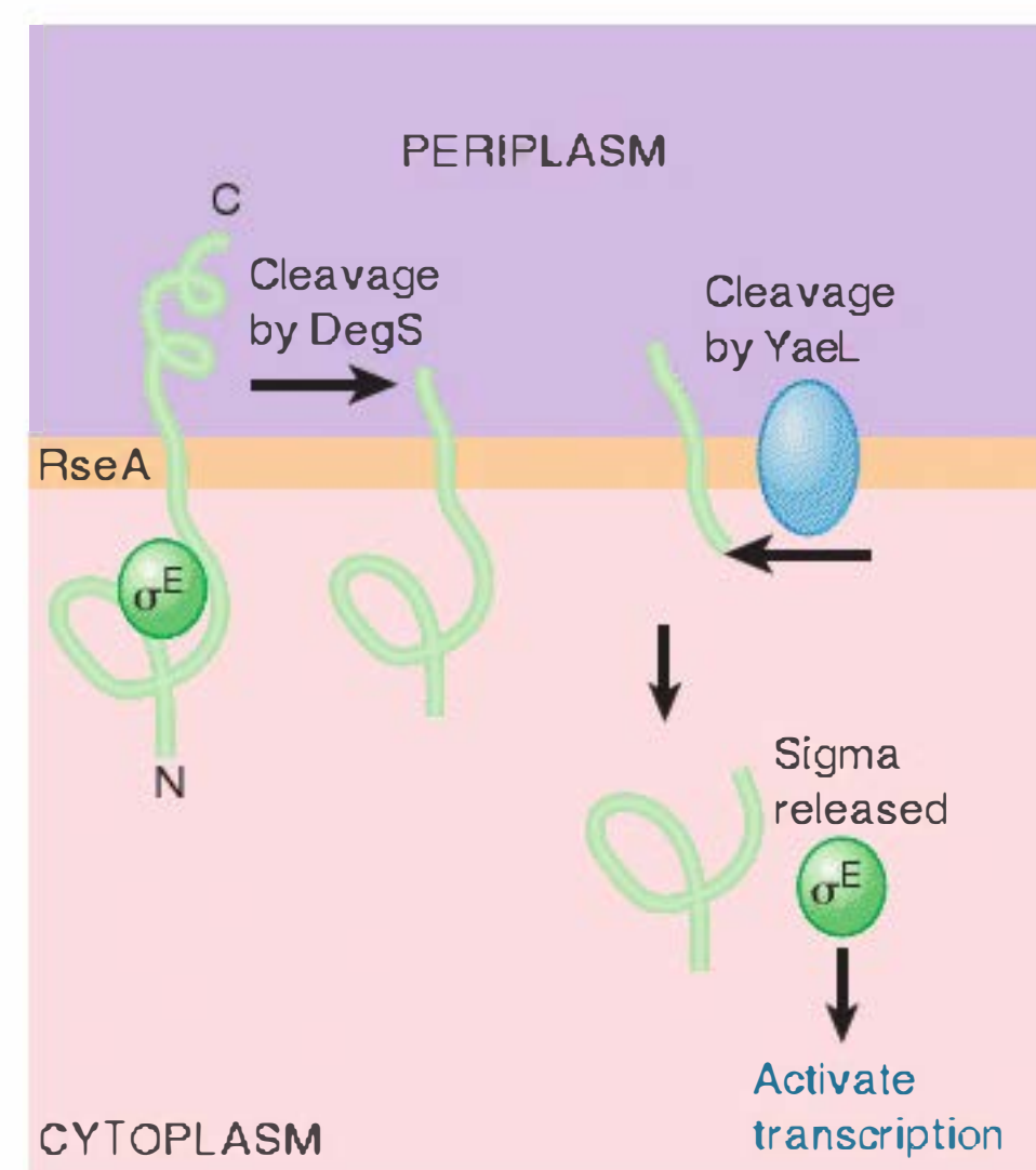
FIGURE 19.38 RseA is synthesized as a protein in the inner membrane. Its cytoplasmic domain binds the \sigma^E factor. RseA is cleaved sequentially in the periplasmic space and then in the cytoplasm. The cytoplasmic cleavage releases \sigma^E .
