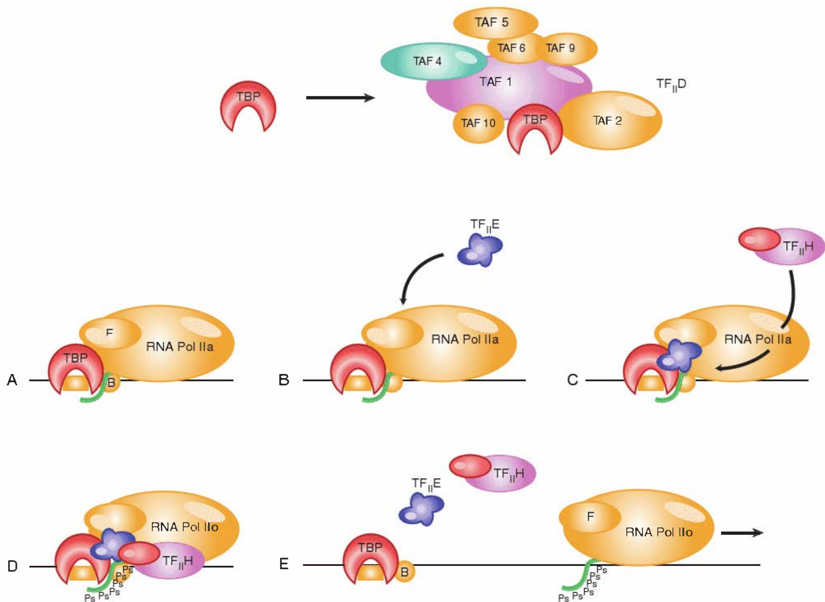
FIGURE 20.11 An initiation complex assembles at promoters for RNA polymerase II by an ordered sequence of association with transcription factors. TF II D consists of TBP plus its associated TAFs as shown in the top panel; TBP alone, rather than TF II D, is shown in the remaining panels for simplicity. Adapted from M. E. Maxon, J. A. Goodrich, and R. Tijan, Genes Dev. 8 (1994): 515–524.
