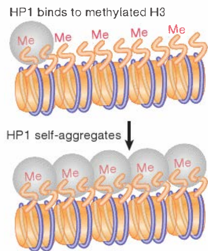
FIGURE 29.7 Binding of HP1 to methylated histone H3 forms a trigger for silencing because further molecules of HP1 aggregate along the methylation chromatin domain.
