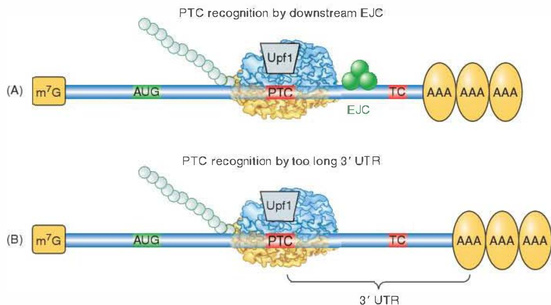
FIGURE 22.14 Two mechanisms by which a termination codon is recognized as premature. (A) In mammals, the presence of an EJC downstream of a termination codon targets the mRNA for NMD. (B) In probably all eukaryotes, an abnormally long 3' UTR is recognized by the distance between the termination codon and the poly(A)-PABP complex. In either case, the Upf1 protein binds to the terminating ribosome to trigger decay.
