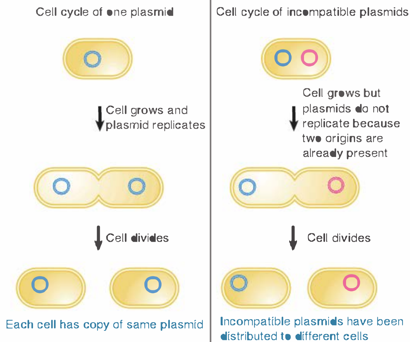
FIGURE 14.16 Two plasmids are incompatible (they belong to the same compatibility group) if their origins cannot be distinguished at the stage of initiation. The same model could apply to segregation.
