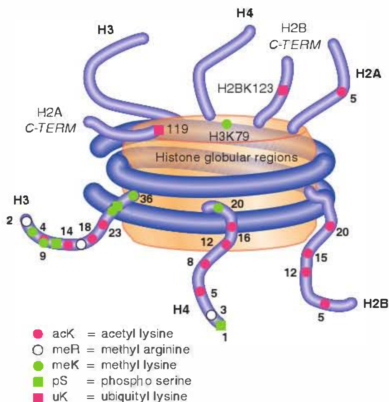
FIGURE 10.16 The histone tails can be acetylated, methylated, phosphorylated, and ubiquitylated at numerous sites. Not all possible modifications are shown. Adapted from The Scientist 17 (2003): p. 27.
