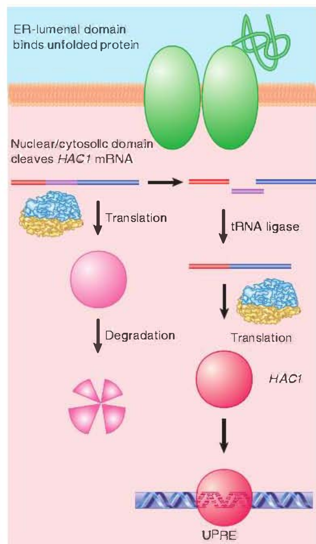
FIGURE 21.39 The unfolded protein response occurs by activating special splicing of HAC1 mRNA to produce a transcription factor that recognizes the UPRE.
