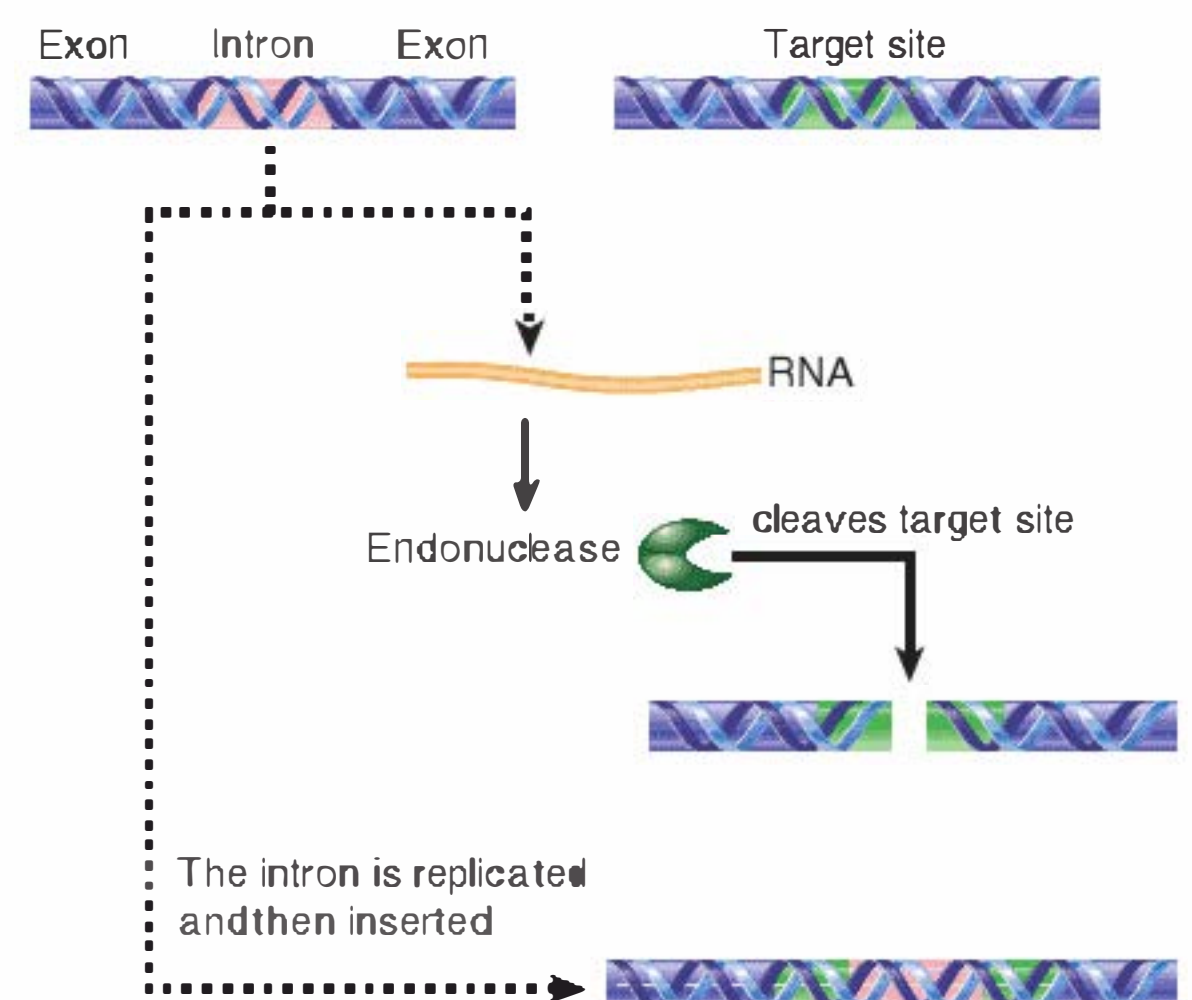
FIGURE 23.11 An intron encodes an endonuclease that makes a double-strand break in DNA. The sequence of the intron is duplicated and then inserted at the break.
