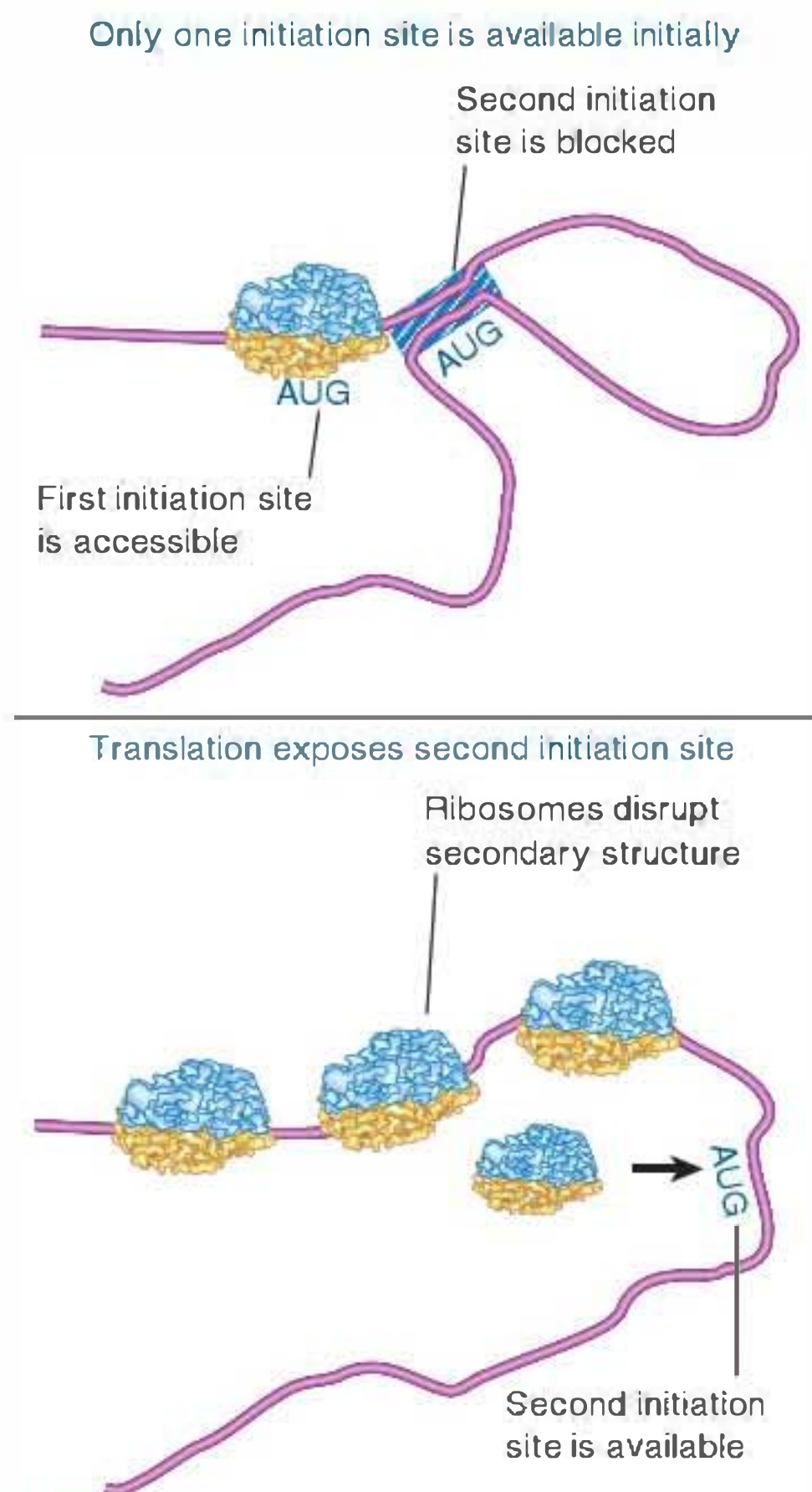
FIGURE 24.52 Secondary structure can control initiation. Only one initiation site is available in the RNA phase, but translation of the first cistron changes the conformation of the RNA so that other initiation site(s) become available.
