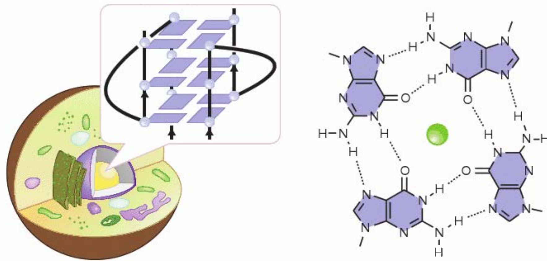
FIGURE 30.15 G-quartet and G-quadruplex structures and topologies. The guanine bases are connected by Hoogsteen hydrogen-bonded base pairing. A central monovalent ion is necessary for formation and stabilization. Reprinted from Yan Xu, et al., Proc. Natl. Acad. Sci. USA 107 (2010): 14579–14584. Copyright © 2010 National Academy of Sciences, U.S.A.
