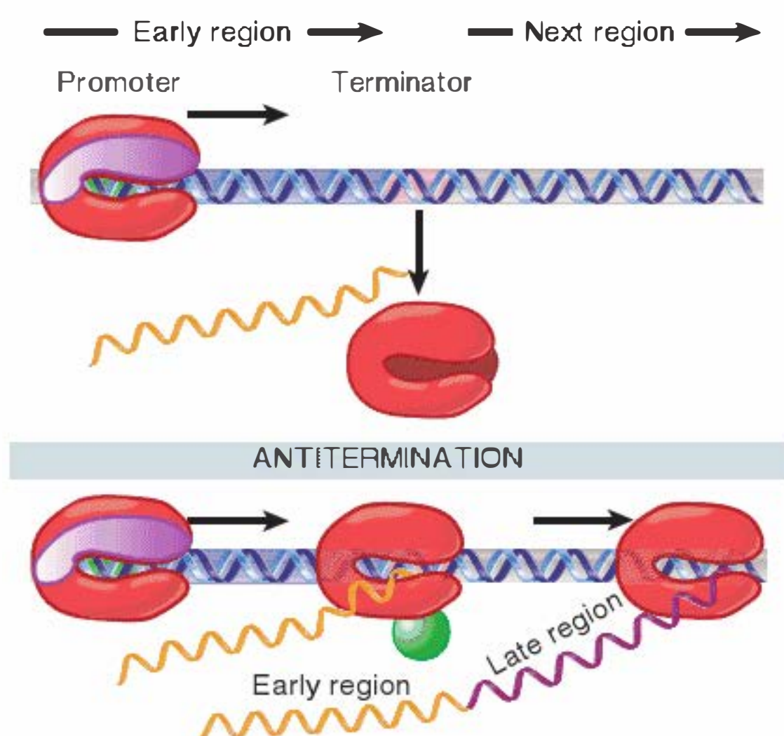
FIGURE 27.5 Control at termination requires adjacent units, so that transcription can read from the first gene into the next gene. This produces a single mRNA that contains both sets of genes.
