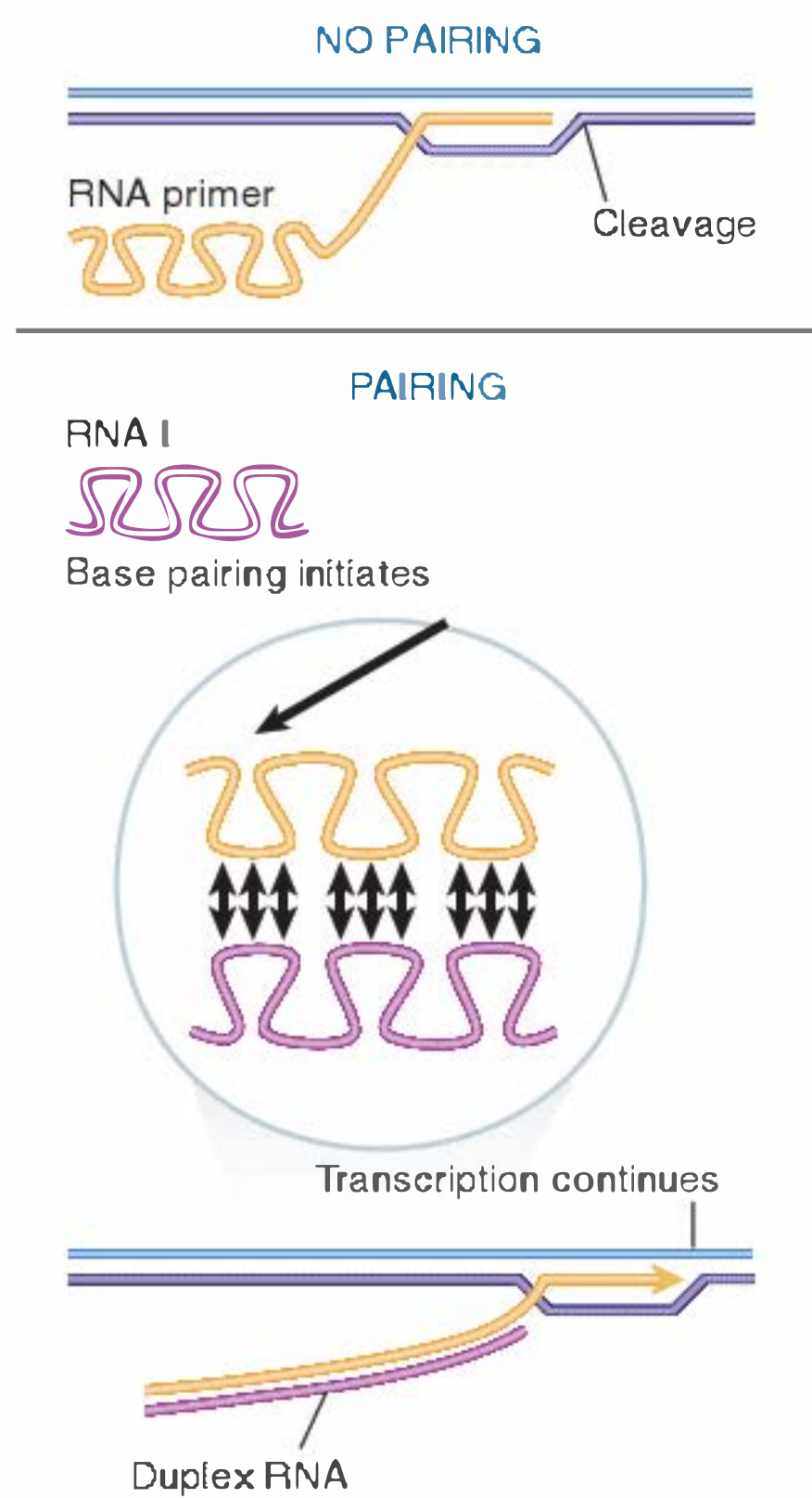
FIGURE 14.19 Base pairing with RNA I may change the secondary structure of the primer RNA sequence and thus prevent cleavage from generating a 3'-OH end.
