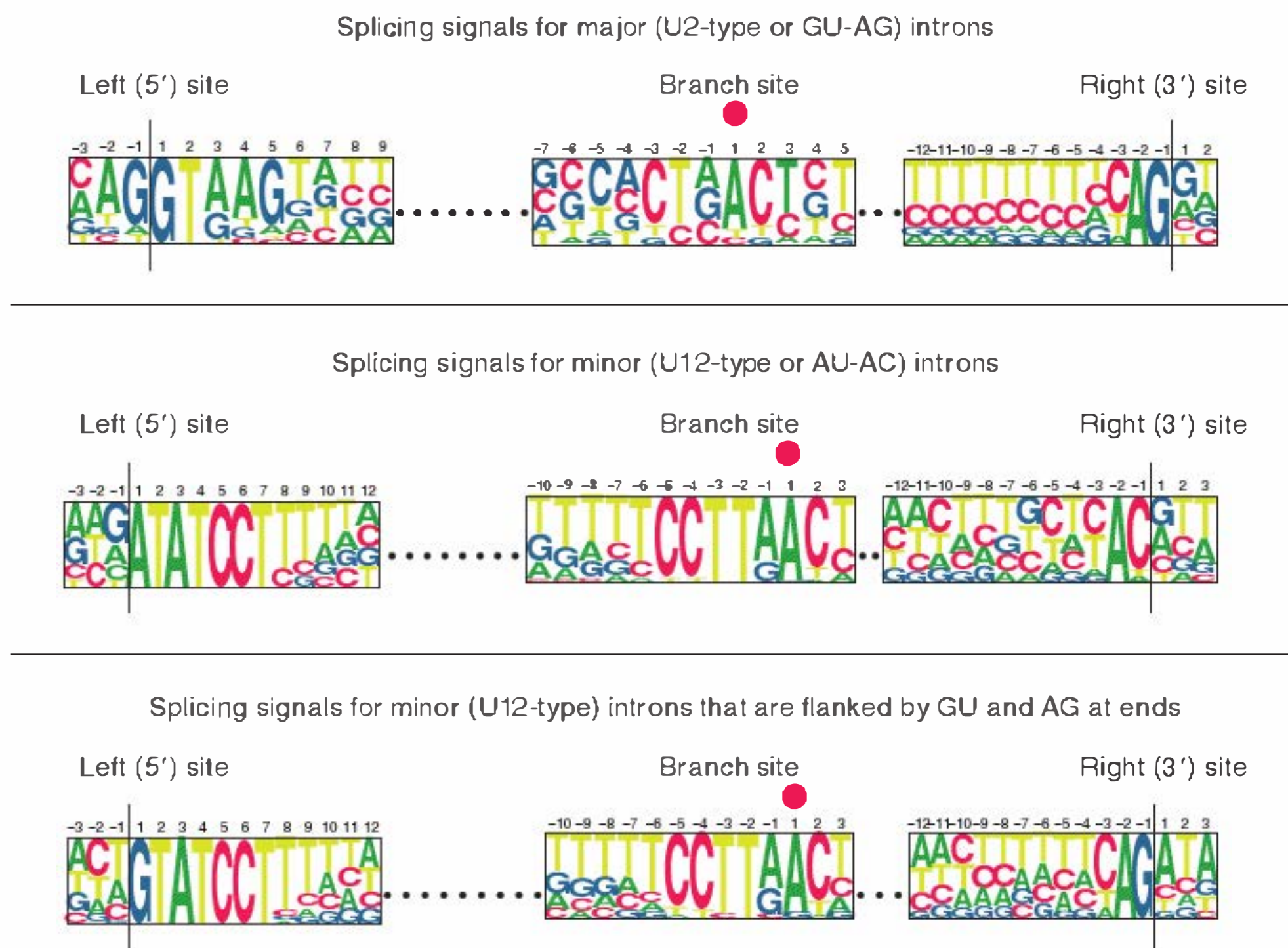
FIGURE 21.3 The ends of nuclear introns are defined by the GU-AG rule (shown here as GT-AG in the DNA sequence of the gene). Minor introns are defined by different consensus sequences at the 5' splice site, branch site, and 3' splice site.
