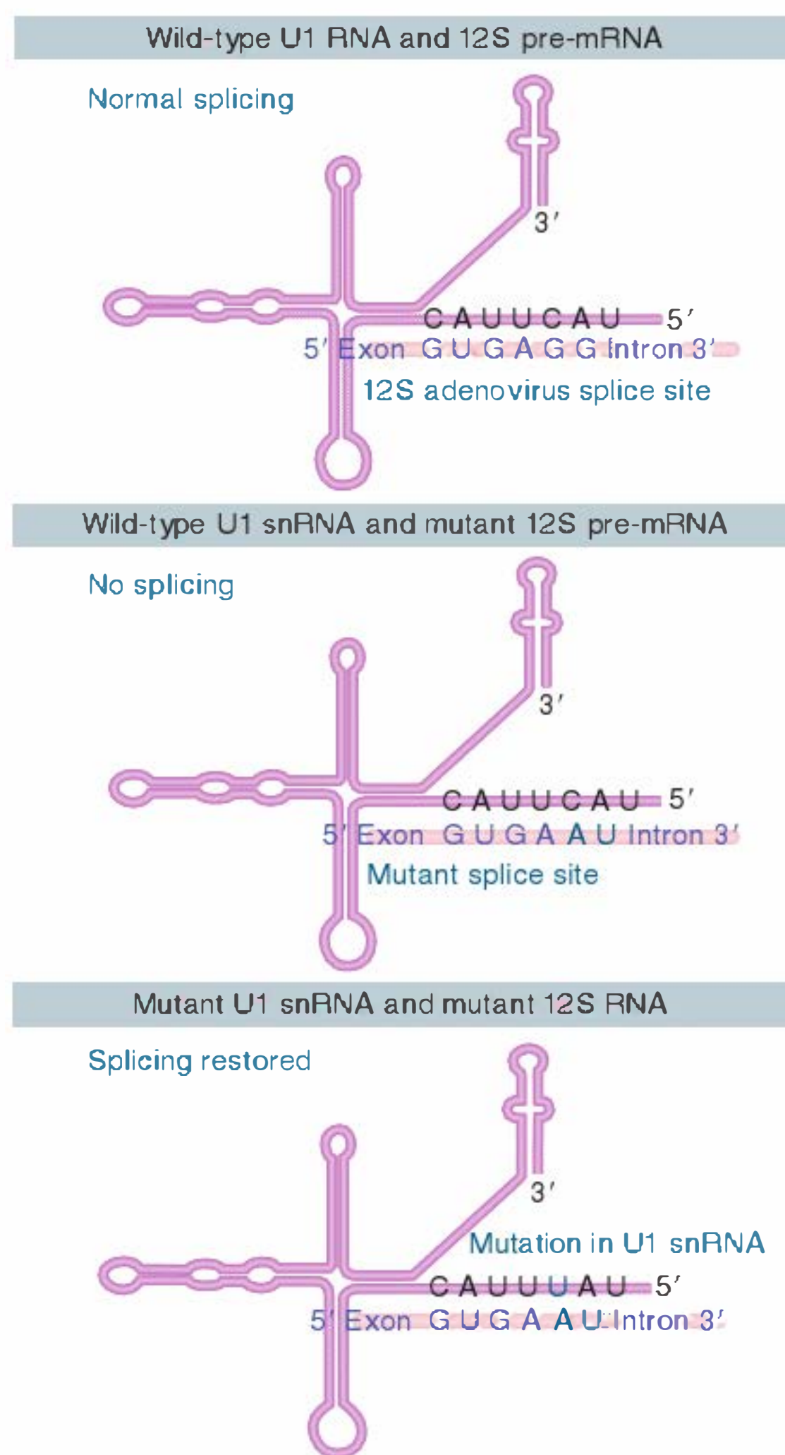
FIGURE 21.9 Mutations that abolish function of the 5′ splice site can be suppressed by compensating mutations in U1 snRNA that restore base pairing.
