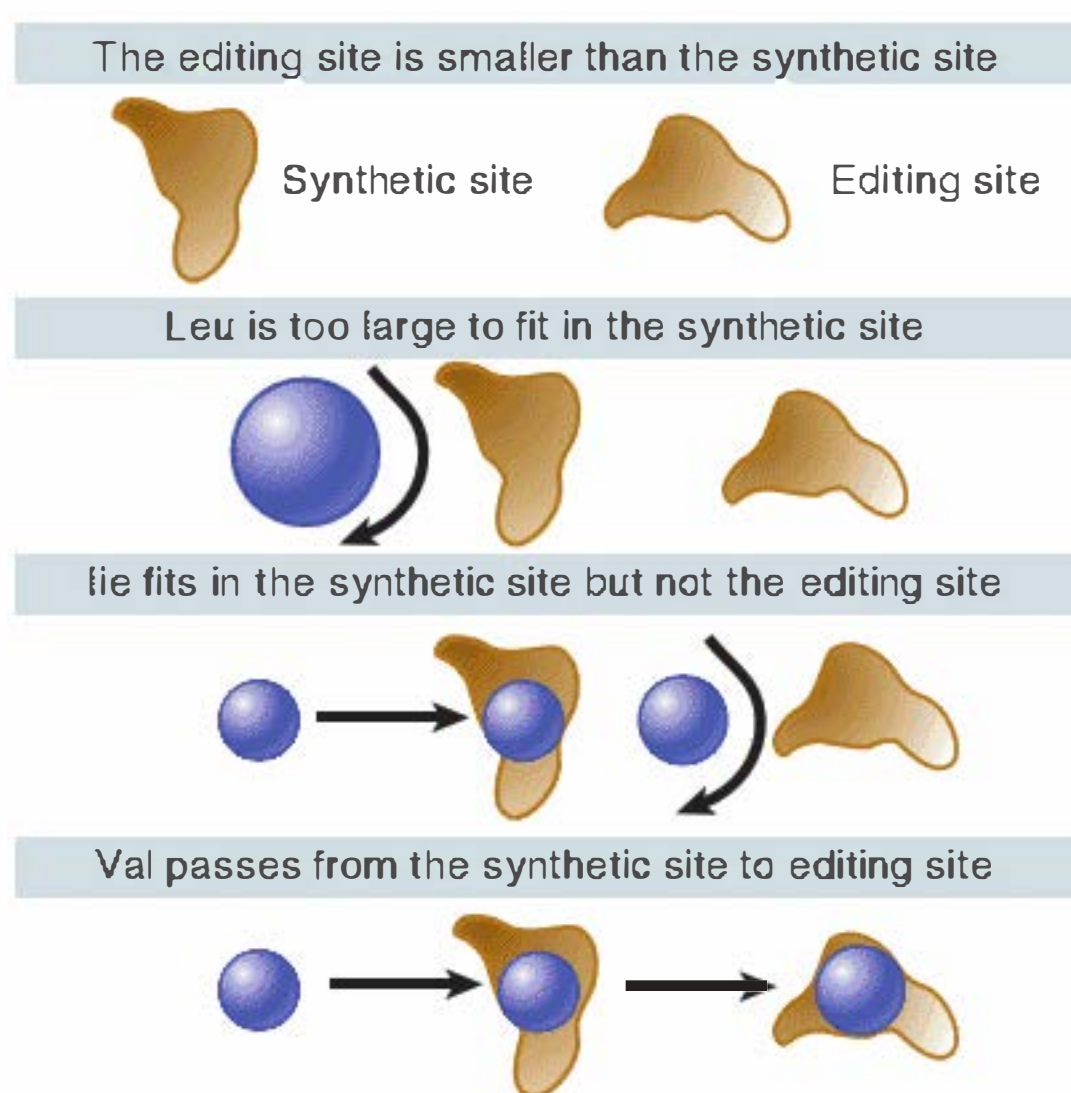
FIGURE 25.19 Isoleucyl-tRNA synthetase has two active sites. Amino acids larger than Ile cannot be activated because they do not fit in the synthetic site. Amino acids smaller than Ile are removed because they are able to enter the editing site.
