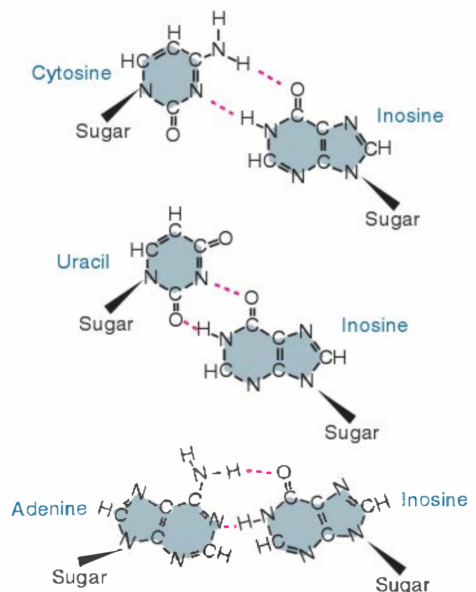
FIGURE 25.8 Inosine can pair with any U, C, or A.
