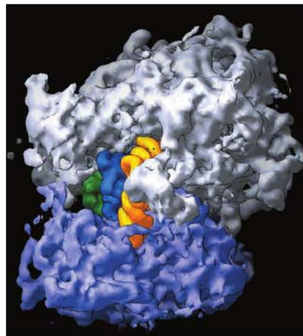
FIGURE 24.43 The 70S ribosome consists of the 50S subunit (white) and the 30S subunit (purple), with three tRNAs located superficially: yellow in the A site, blue in the P site, and green in the E site. Photo courtesy of Harry Noller, University of California, Santa Cruz.
