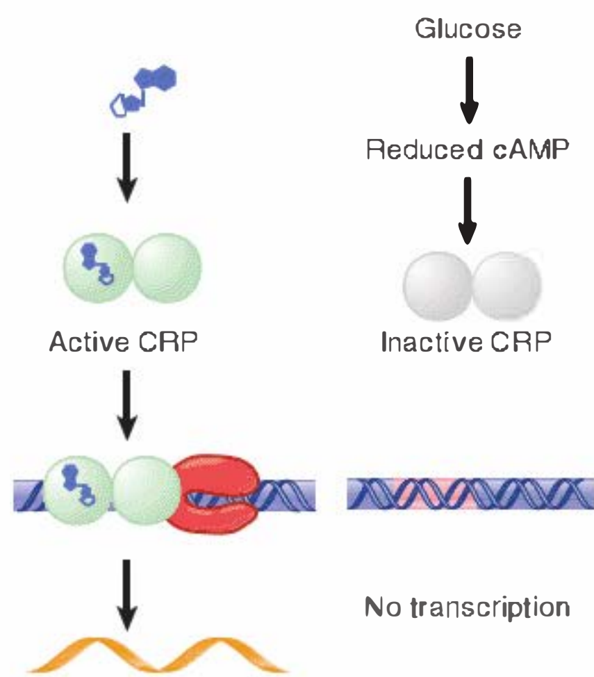
FIGURE 26.27 By reducing the level of cyclic AMP, glucose inhibits the transcription of operons that require CRP activity.
