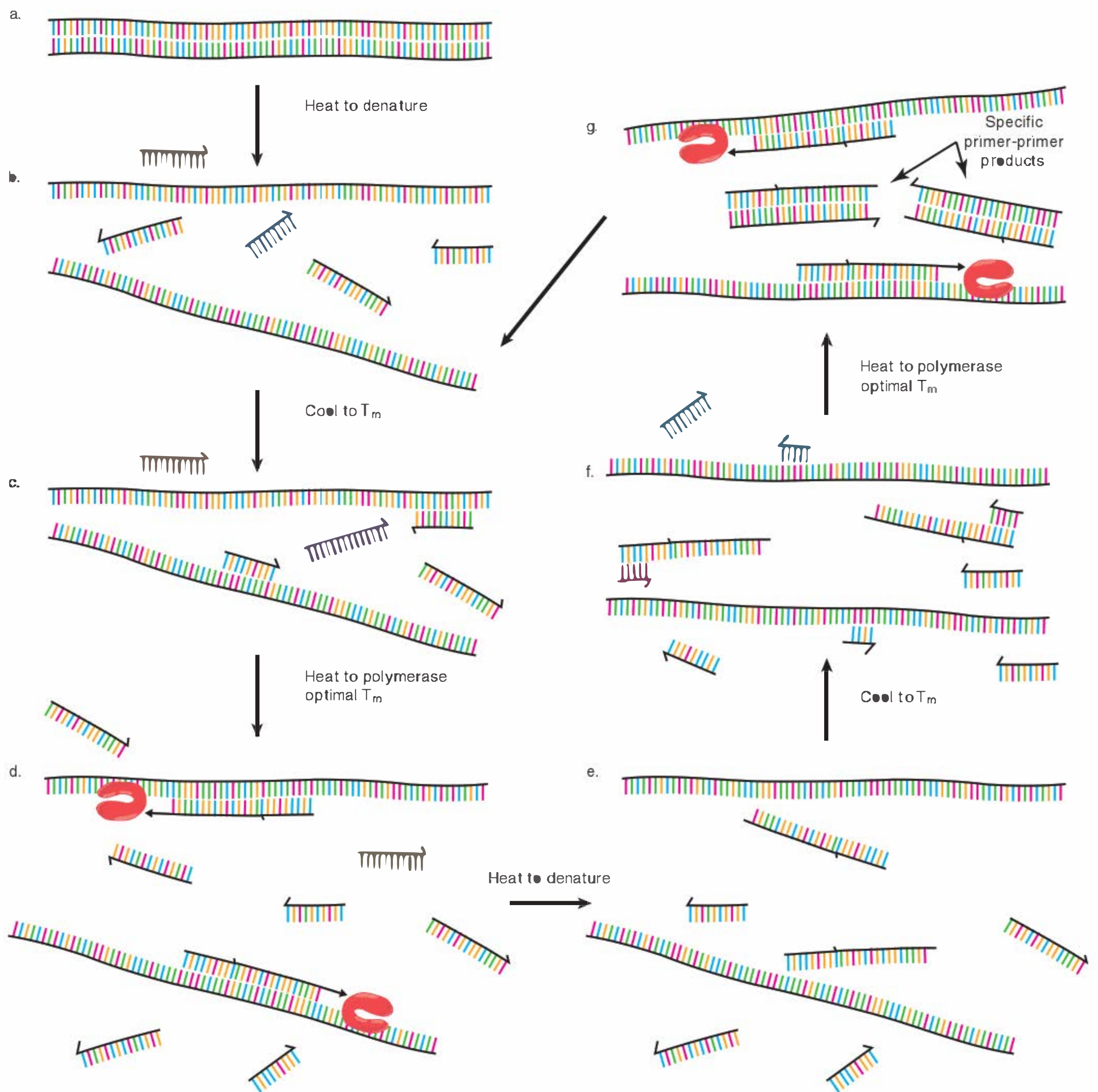
FIGURE 3.19 Thermally driven cycles of primer extension where primers of opposite polarity have nearby priming sites on each of the two template strands leads to the exponential production of the short, primer-to-primer-defined sequence (the “amplicon”).
