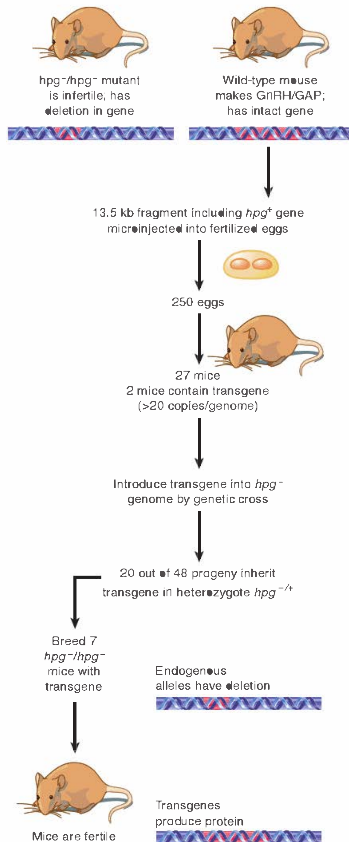
FIGURE 3.28 Hypogonadism can be averted in the progeny of hpg mice by introducing a transgene that has the wild-type sequence.
