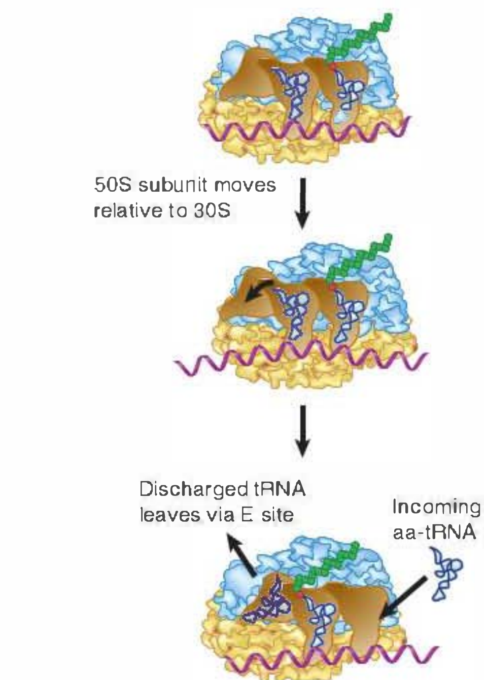
FIGURE 24.29 Models for translocation involve two stages. First, at peptide bond formation the aminoacyl end of the tRNA in the A site becomes relocated in the P site. Second, the anticodon end of the tRNA becomes relocated in the P site.
