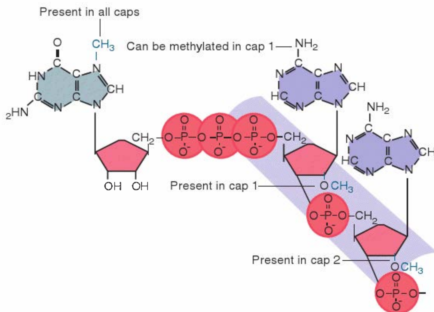
FIGURE 21.2 The cap blocks the 5' end of mRNA and can be methylated at several positions.
