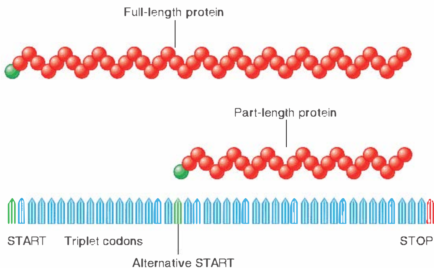
FIGURE 4.12 Two proteins can be generated from a single gene by starting (● terminating) expression at different points.
