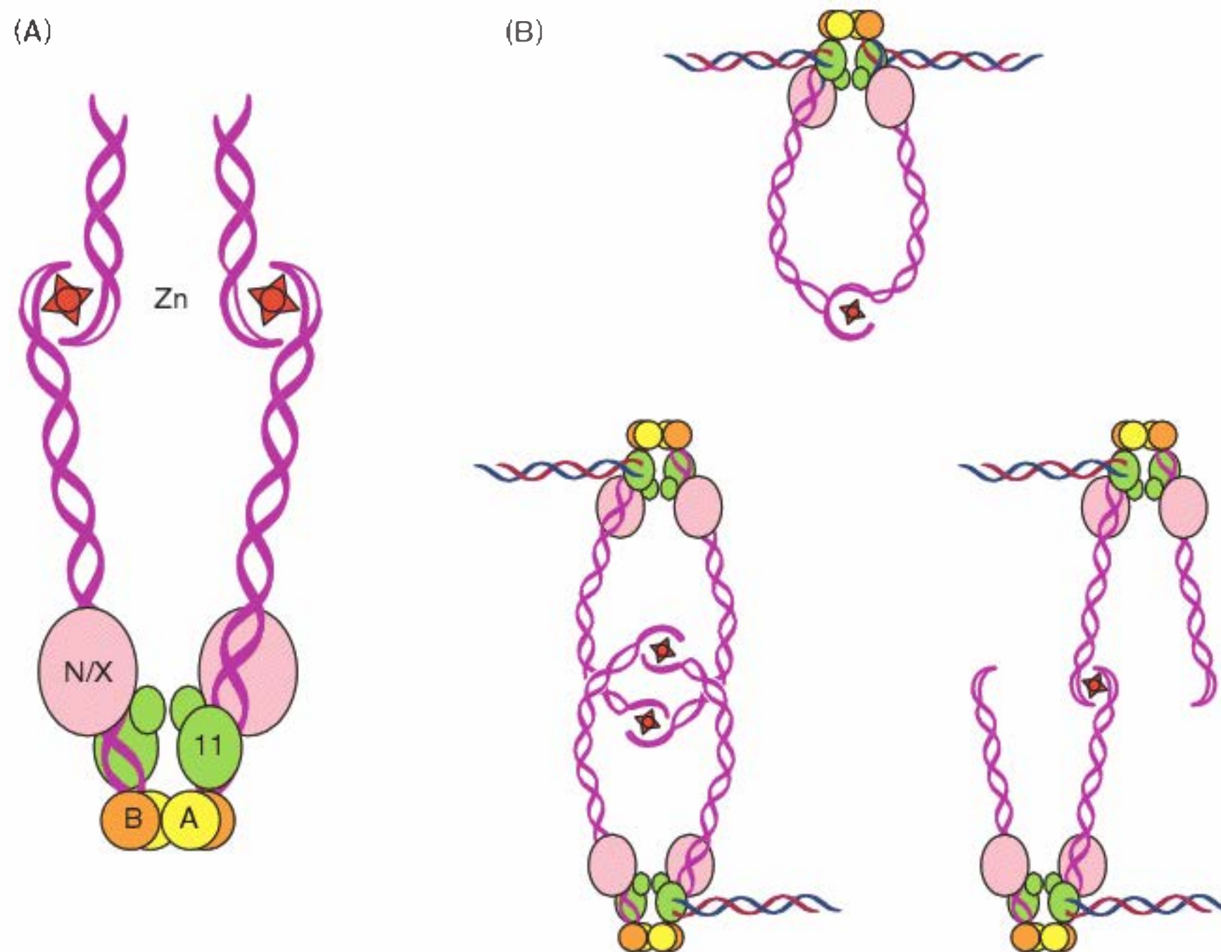
FIGURE 15.22 Structure of Rad50 and model for the MRN/X complex binding to double-strand breaks. Rad50 has a coiled coil domain similar to SMC proteins. The globular end contains two ATP-binding and hydrolysis regions (A and B) and forms a complex with Mre11 and Nbs1 (N) or Xrs2 (X). The other end of the coil binds zinc cation and forms a dimer with another MRN/X molecule. The globular end binds to chromatin. The complex binds to double-strand breaks and can bring them together in a reaction involving two ends and one MRN/X complex (top right figure) or through an interaction between two MRN/X dimers (bottom right figure). Adapted from M. Lichten, Nat. Struct. Mol. Biol. 12 (2005): 392–393.
