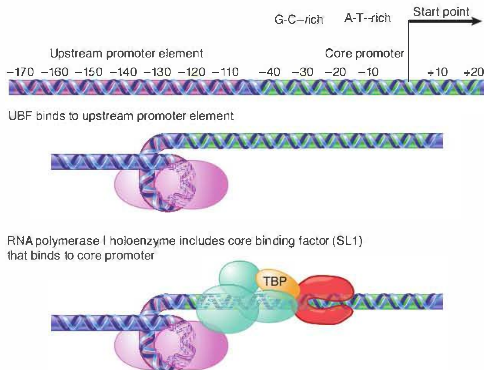
FIGURE 20.3 Transcription units for RNA polymerase I have a core promoter separated by \sim 70 bp from the upstream promoter element. UBF binding to the UPE increases the ability of core-binding factor to bind to the core promoter. Core-binding factor (SL1) positions RNA polymerase I at the start point.
