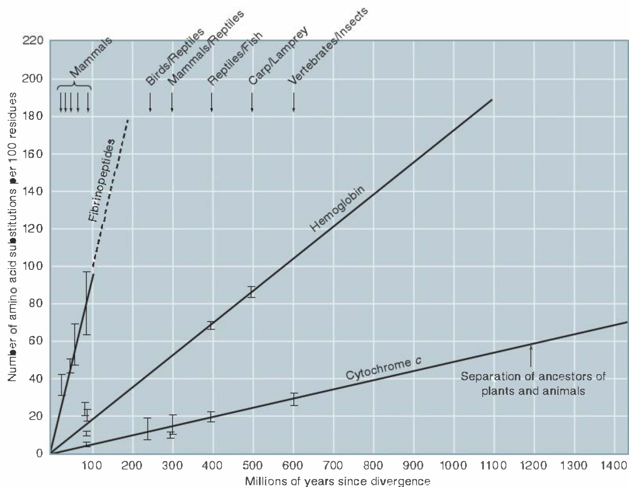
FIGURE 8.7 The rate of evolution of three types of proteins over time. The approximately constant rate of evolution of each protein type is a molecular clock. Reproduced with kind permission from Springer Science+Business Media: J. Mol. Evol. , The structure of cytochrome and the rates of molecular evolution, vol. 1, 1971, pp. 26–45, R. E. Dickerson, fig. 3. Courtesy of Richard Dickerson, University of California, Los Angeles.
