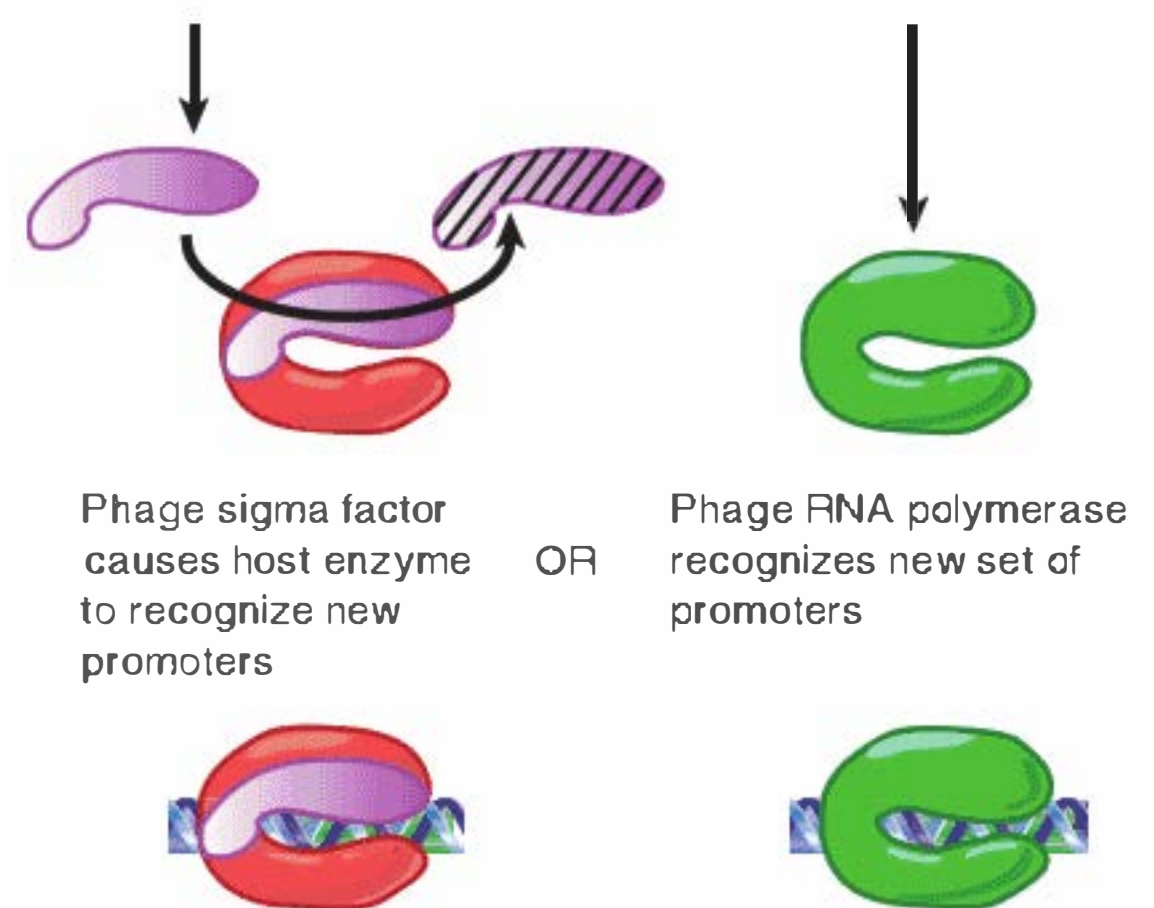
FIGURE 27.6 A phage may control transcription at initiation either by synthesizing a new sigma factor that replaces the host sigma factor or by synthesizing a new RNA polymerase.
