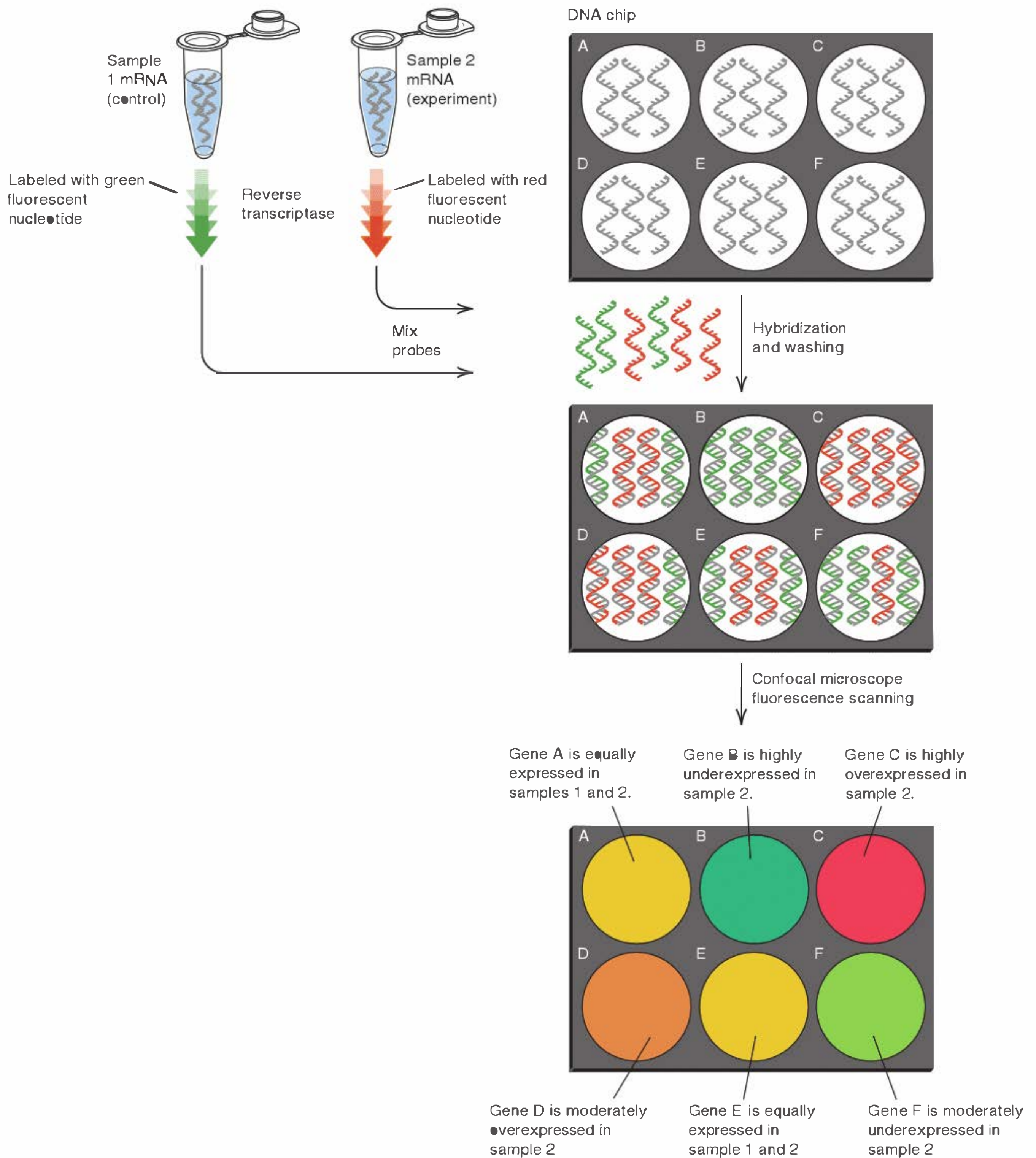
FIGURE 3.25 Gene expression arrays are used to detect the levels of all the expressed genes in an experimental sample. mRNAs are isolated from control and experimental cells or tissues and reverse transcribed in the presence of fluorescently labeled nucleotides (or primers), resulting in labeled cDNAs with different fluorophores (red and green strands) for each sample. Competitive hybridization of the red and green cDNAs to the microarray is proportional to the relative abundance of each mRNA in the two samples. The relative levels of red and green fluorescence are measured by microscopic scanning and are displayed as a single color. Red or orange indicates increased expression in the red (experimental) sample, green or yellow-green indicates lower expression, and yellow indicates equal levels of expression in the control and experiment.
