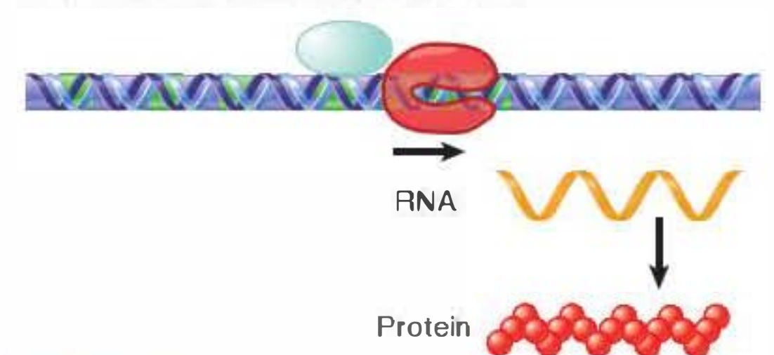
FIGURE 26.3 In positive control, a trans -acting factor must bind to the cis -acting site in order for RNA polymerase to initiate transcription at the promoter.
