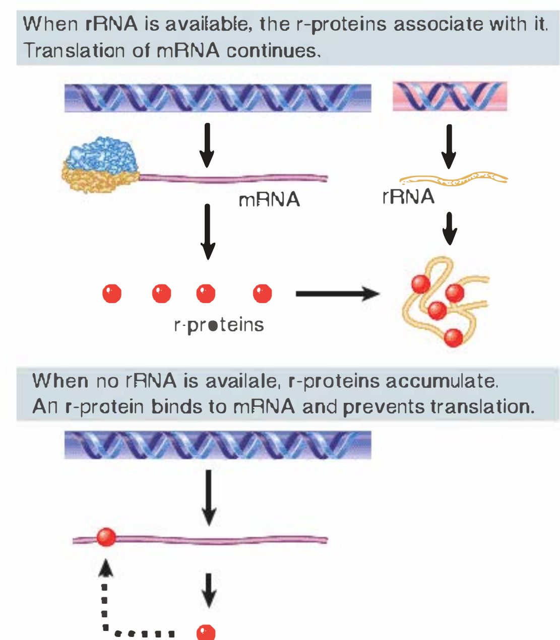
FIGURE 26.42 Translation of the r-protein operons is autogenously controlled and responds to the level of rRNA.
