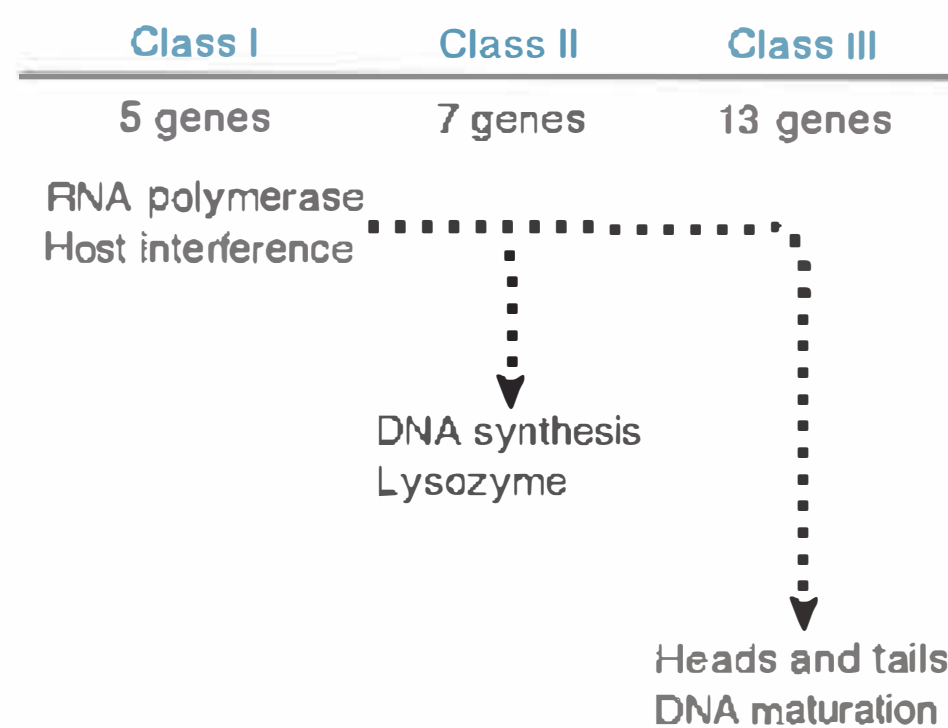
FIGURE 27.7 Phage T7 contains three classes of genes that are expressed sequentially. The genome is ~38 kb.
