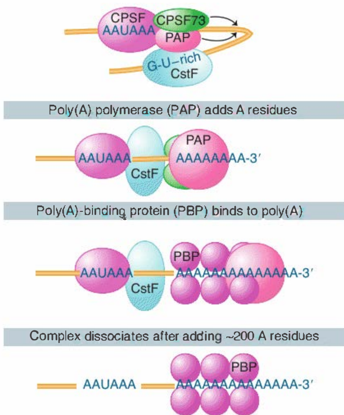
FIGURE 21.30 The 3' processing complex consists of several activities. CPSF and CstF each consist of several subunits; the other components are monomeric. The total mass is >900 kD.
