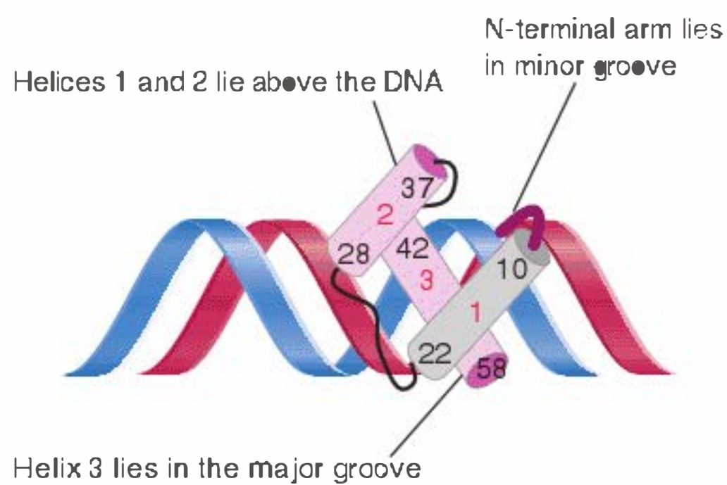
FIGURE 28.14 Helix 3 of the homeodomain binds in the major groove of DNA, with helices 1 and 2 lying outside the double helix. Helix 3 contacts both the phosphate backbone and specific bases. The N-terminal arm lies in the minor groove and makes additional contacts.
