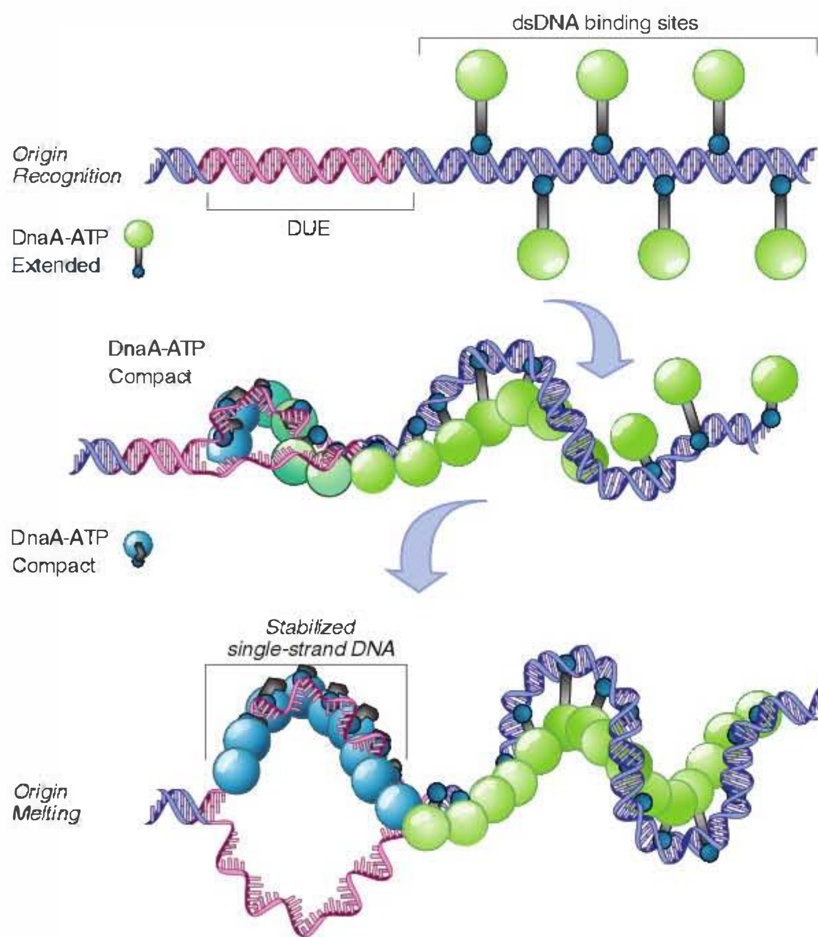
FIGURE 12.9 A two-state assembly model during initiation. DnaA-ATP monomers in an extended state associate with the high-affinity 13-mer sequences. DnaA-ATP transitions to a compact state as the 9-mer region begins to melt, stabilizing the single-stranded DNA. Adapted from Journal of Biological Chemistry , vol.285, Karl E. Duderstadt, et al., Origin Remodeling and Opening in Bacteria..., pp. 28229–28239. © 2010 The American Society for Biochemistry and Molecular Biology.
