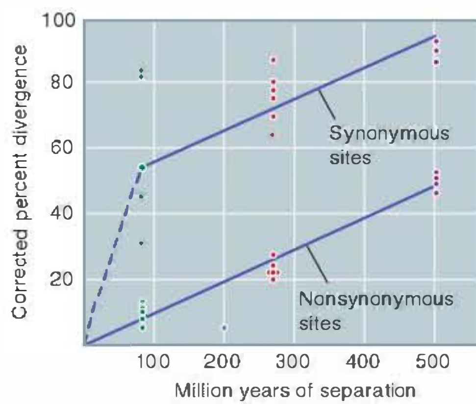
FIGURE 8.8 Divergence of DNA sequences depends on evolutionary separation. Each point on the graph represents a pairwise comparison.
