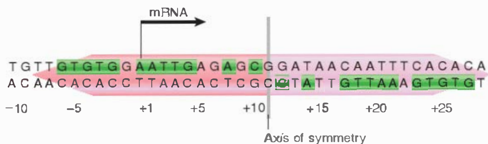
FIGURE 26.17 The lac operator has a symmetrical sequence. The sequence is numbered relative to the start point for transcription at +1. The pink arrows to the left and to the right identify the two dyad repeats. The green blocks indicate the positions of identity.
