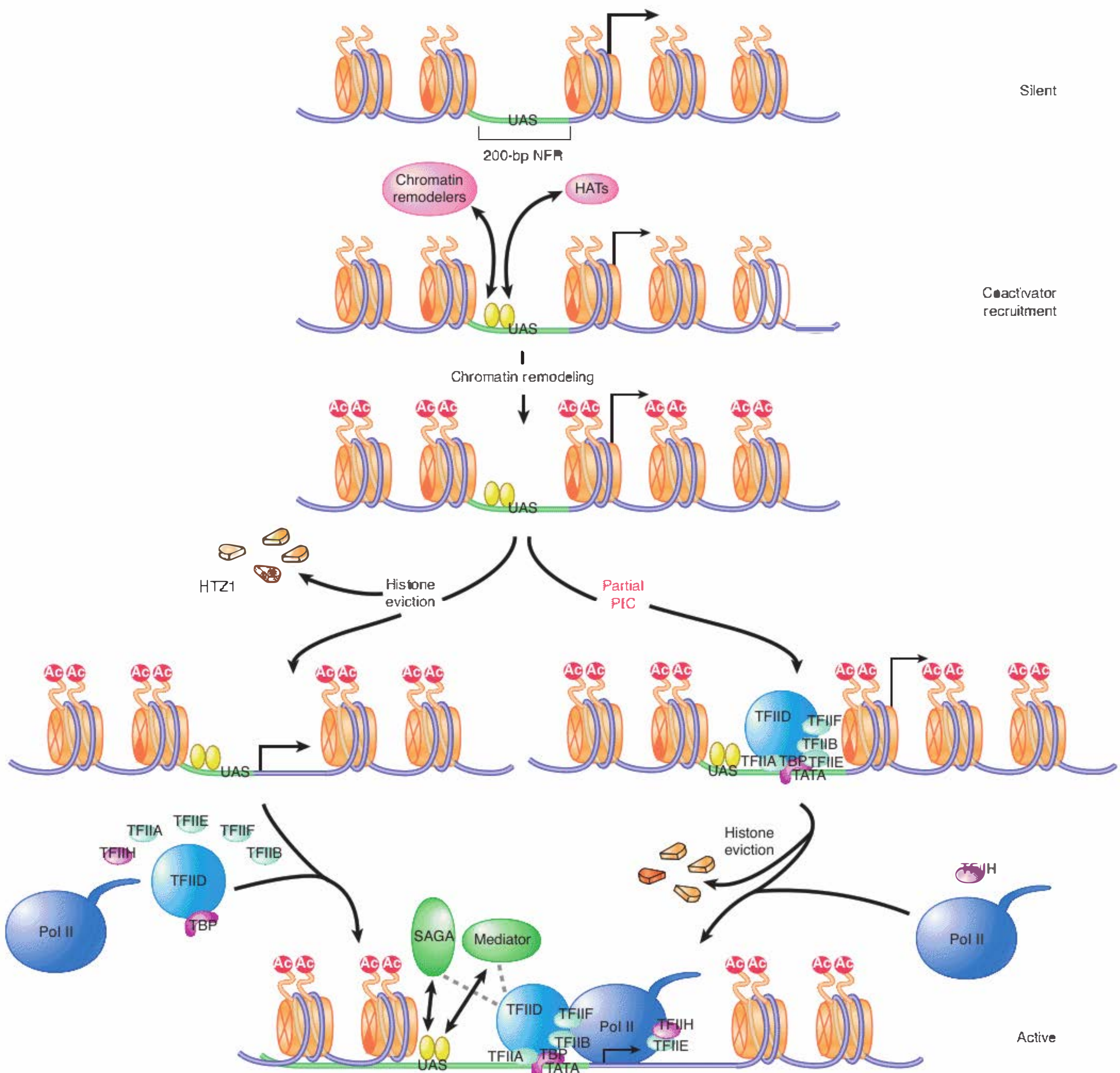
FIGURE 28.29 Htz1-containing nucleosomes flank a 200-bp NFR on both sides of a promoter. Upon targeting to the upstream activation sequence (UAS), activators recruit various coactivators (such as Swi/Snf or SAGA). This recruitment further increases the binding of activators, particularly for those bound within nucleosomal regions. More importantly, histones are acetylated at promoter-proximal regions, and these nucleosomes become much more mobile. In one model (left), a combination of acetylation and chromatin remodeling directly results in the loss of Htz1-containing nucleosome, thereby exposing the entire core promoter to the GTFs and Pol II. SAGA and Mediator then facilitate PIC formation through direct interactions. In the other model (right), which represents the remodeled state, partial PICs could be assembled at the core promoter without loss of Htz1. It is the binding of Pol II and TFIID that leads to the displacement of Htz1-containing nucleosomes and the full assembly of PIC. Reprinted from Cell , vol. 128, B. Li, M. Carey, and J. L. Workman, The Role of Chromatin during Transcription , pp. 707–719. Copyright 2007, with permission from Elsevier [ http://www.sciencedirect.com/science/journal/00928674 ].
