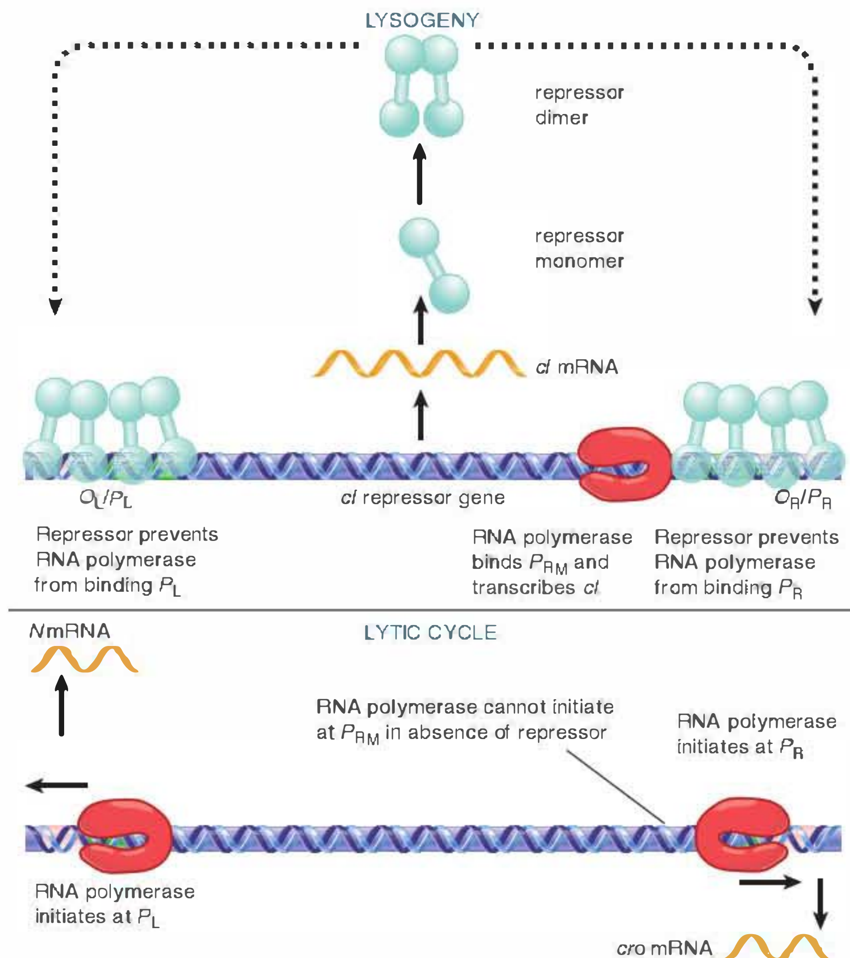
FIGURE 27.27 Lysogeny is maintained by an autoregulatory circuit.
