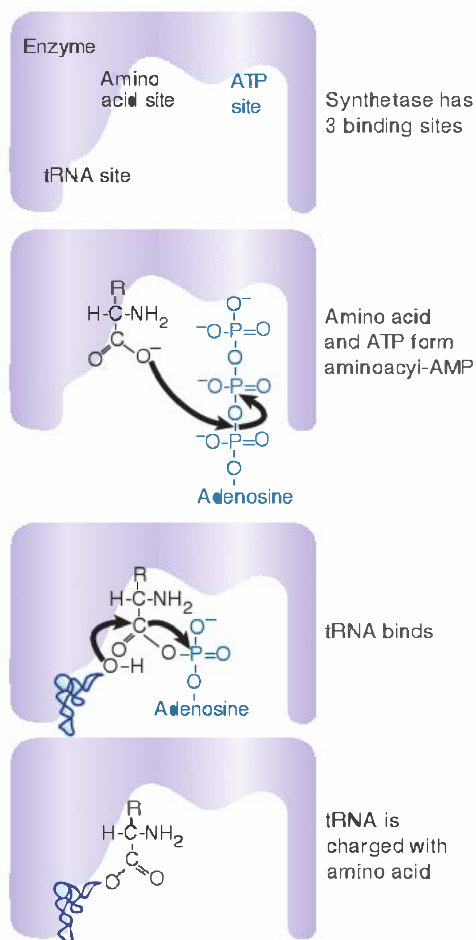
FIGURE 25.13 An aminoacyl-tRNA synthetase charges tRNA with an amino acid.
