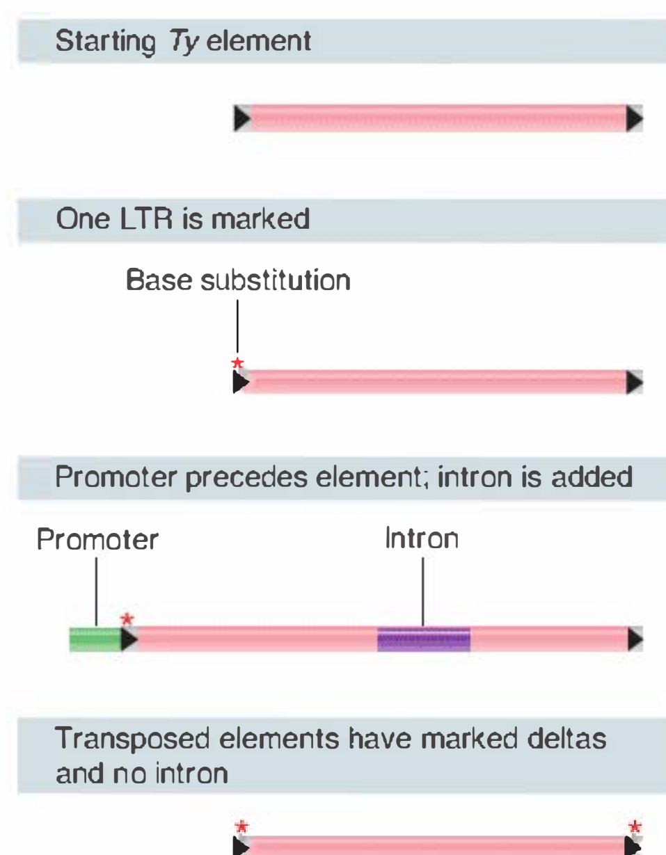
FIGURE 17.34 A unique Ty element, engineered to contain an intron, transposes to give copies that lack the intron. The copies possess identical terminal repeats, which are generated from one of the termini of the original Ty element.
