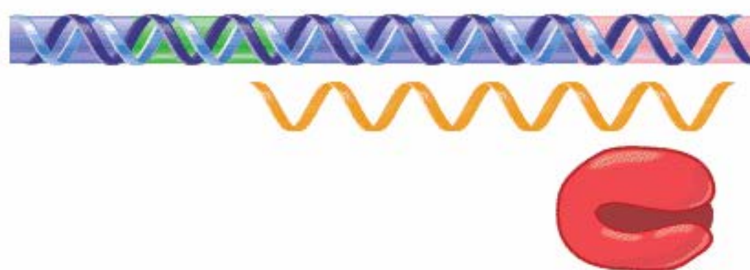
FIGURE 19.6 Transcription has three stages: The enzyme binds to the promoter and melts DNA and remains stationary during initiation; moves along the template during elongation; and dissociates at termination.
