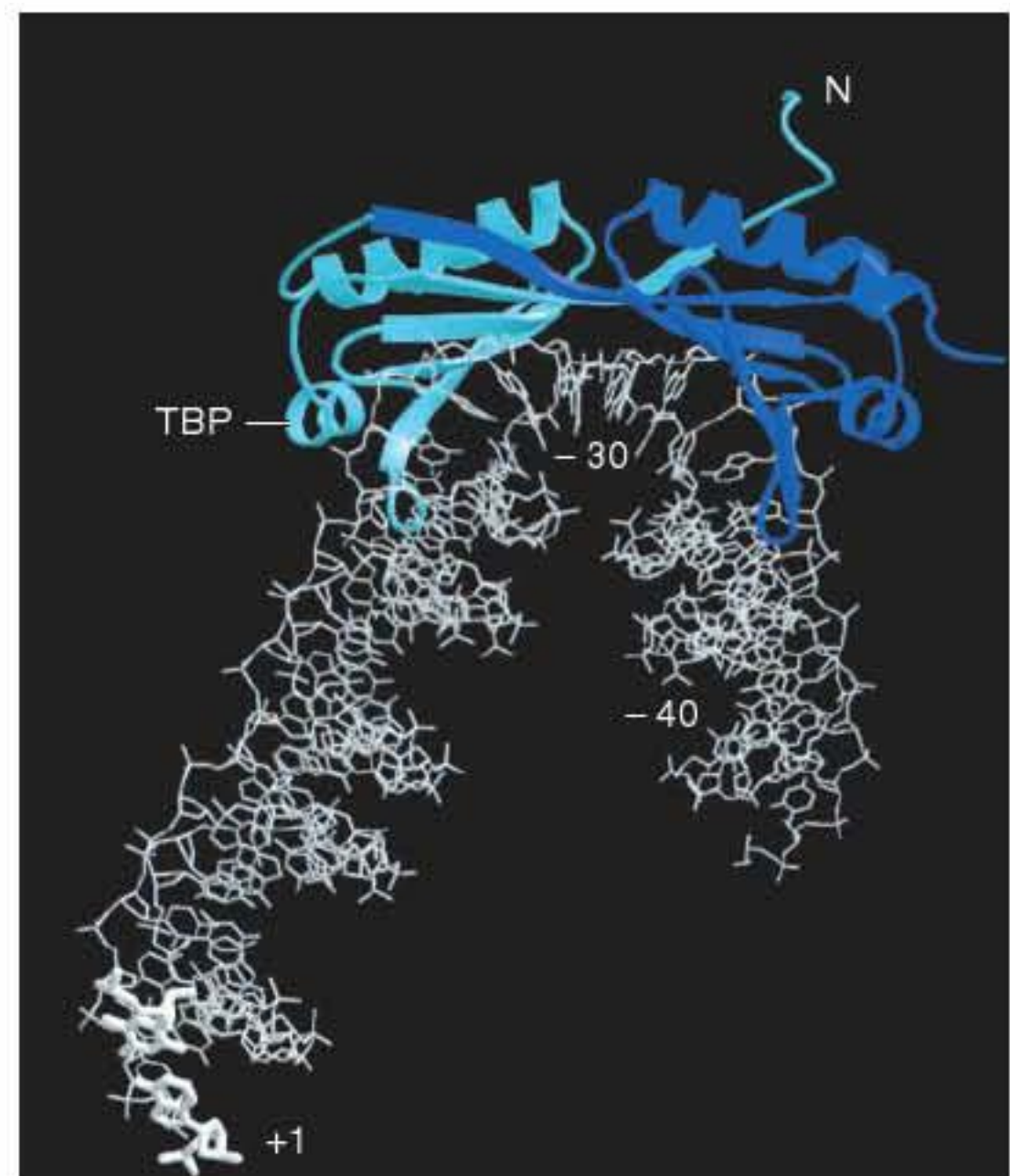
FIGURE 20.10 The cocystal structure of TBP with DNA from -40 to the start point shows a bend at the TATA box that widens the narrow groove where TBP binds. Photo courtesy of Stephen K. Burley.
