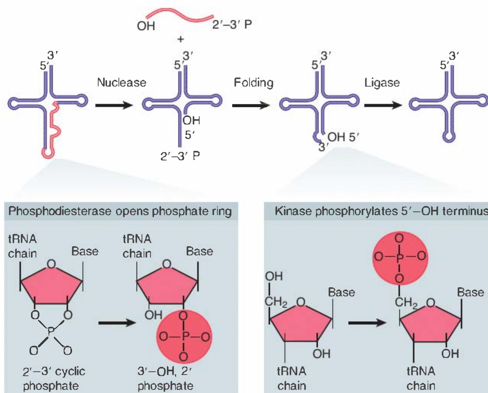
FIGURE 21.38 Splicing of tRNA requires separate nuclease and ligase activities. The exon-intron boundaries are cleaved by the nuclease to generate 2'-3' cyclic phosphate and 5'-OH termini. The cyclic phosphate is opened to generate 3'-OH and 2' phosphate groups. The 5'-OH is phosphorylated. After releasing the intron, the tRNA half molecules fold into a tRNA-like structure that now has a 3'-OH, 5'-P break. This is sealed by a ligase.
