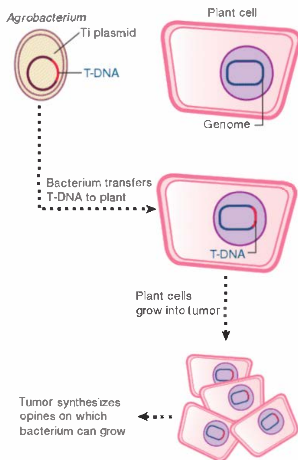
FIGURE 14.25 T-DNA is transferred from Agrobacterium carrying a Ti plasmid into a plant cell, where it becomes integrated into the nuclear genome and expresses functions that transform the host cell.
