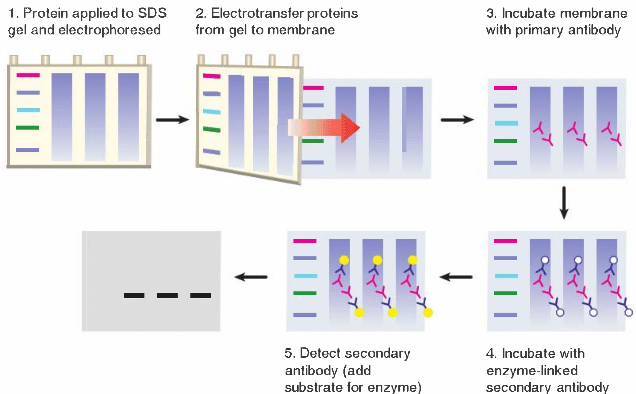
FIGURE 3.24 In a western blot, proteins are separated by size on an SDS gel, transferred to a nitrocellulose membrane, and detected using an antibody. The primary antibody detects the protein and the enzyme-linked secondary antibody detects the primary antibody. The secondary antibody is detected in this example via addition of a chemiluminescent substrate, which results in emission of light that can be detected on X-ray film.
