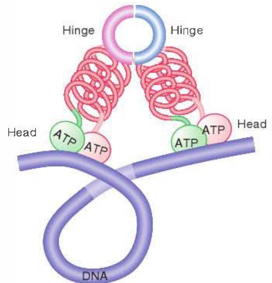
FIGURE 29.18 Condensins may form a compact structure by bending at the hinge, causing DNA to become compacted.
