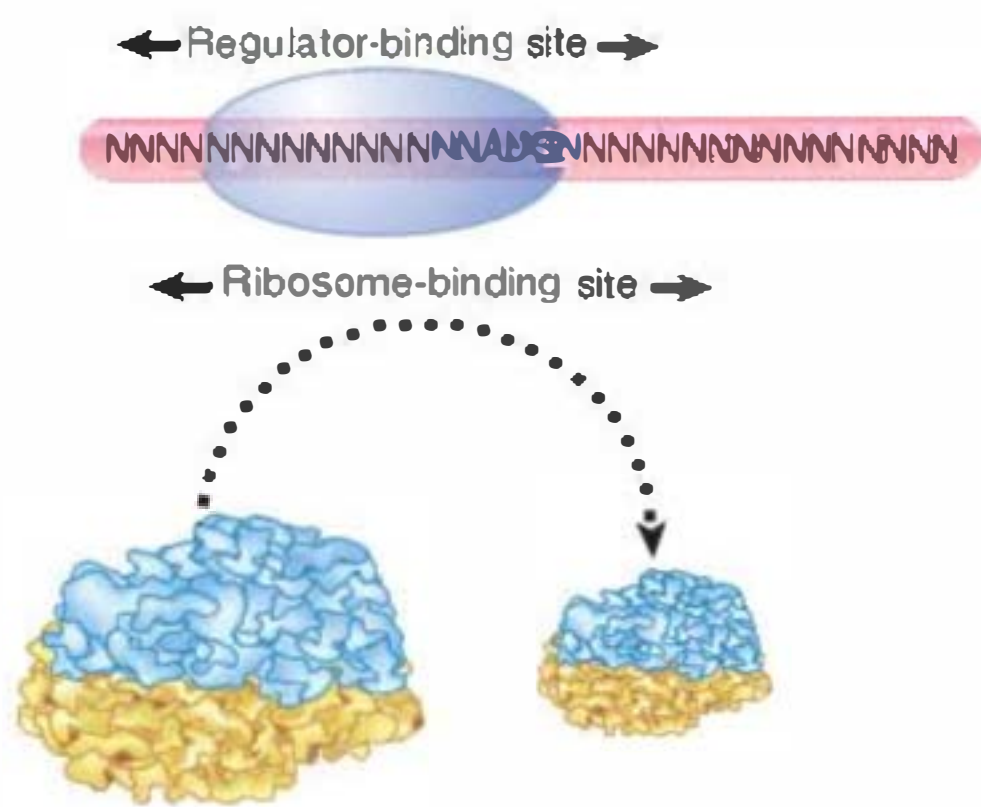
FIGURE 24.50 A regulator protein may block translation by binding to a site on mRNA that overlaps the ribosome-binding site at the initiation codon.
