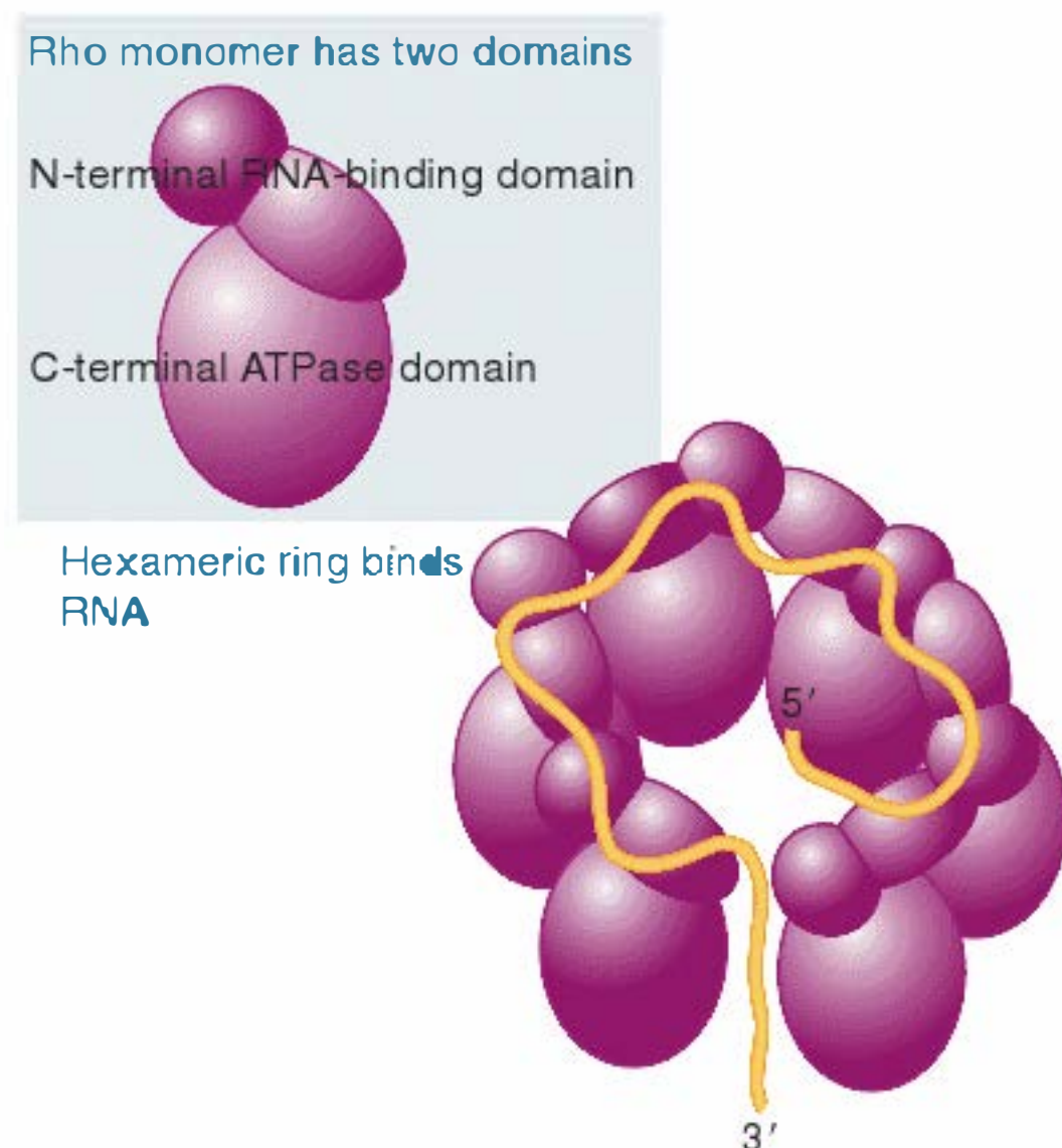
FIGURE 19.32 Rho has an N-terminal, RNA-binding domain and a C-terminal ATPase domain. A hexamer in the form of a gapped ring binds RNA along the exterior of the N-terminal domains. The 5' end of the RNA is bound by a secondary binding site in the interior of the hexamer.
