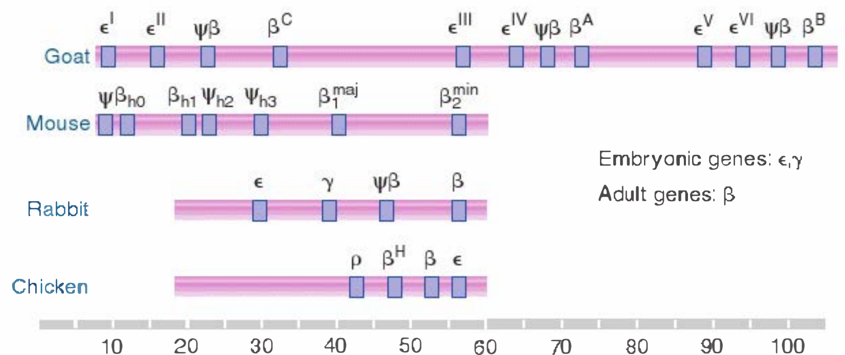
FIGURE 8.22 Clusters of \beta -globin genes and pseudogenes are found in vertebrates. Seven mouse genes include two early embryonic genes, one late embryonic gene, two adult genes, and two pseudogenes. Rabbits and chickens each have four genes.
