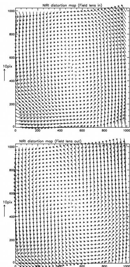
Fig. 3. NIRI distortion maps for images taken with ( top ) or without ( bottom ) the Altair field lens. Arrows indicate the distortions at each position of the detector. For the sake of visibility, we multiplied their length by 10.
