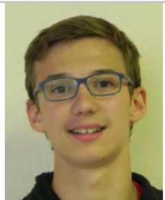
MERLIN Theo
