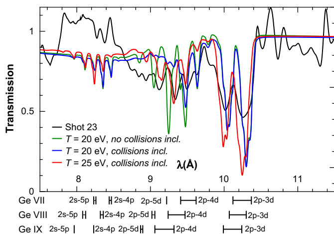
Fig. 10. Experimental transmission of germanium (shot 23) compared with HULLAC calculations, at temperatures of 20 eV and 25 eV, a density of 10 \text{ mg/cm}^3 , and an areal density of 80 \text{ } \mu\text{g/cm}^2 . Only the range 7.5–11.5 Å where structures are found in the computation is plotted. Line identification is proposed for the most abundant ions. (For interpretation of colors in the figure legend, the reader is referred to the web version of the article.)
