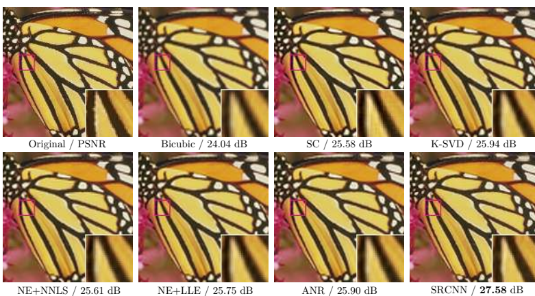
Fig. 8. “Butterfly” image from Set5 with an upscaling factor 3
