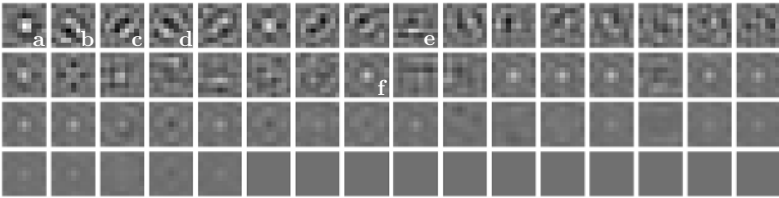
Fig. 5. The figure shows first-layer filters trained on 91 images with an upscaling factor 2. The filters are organized based on their respective variances.
